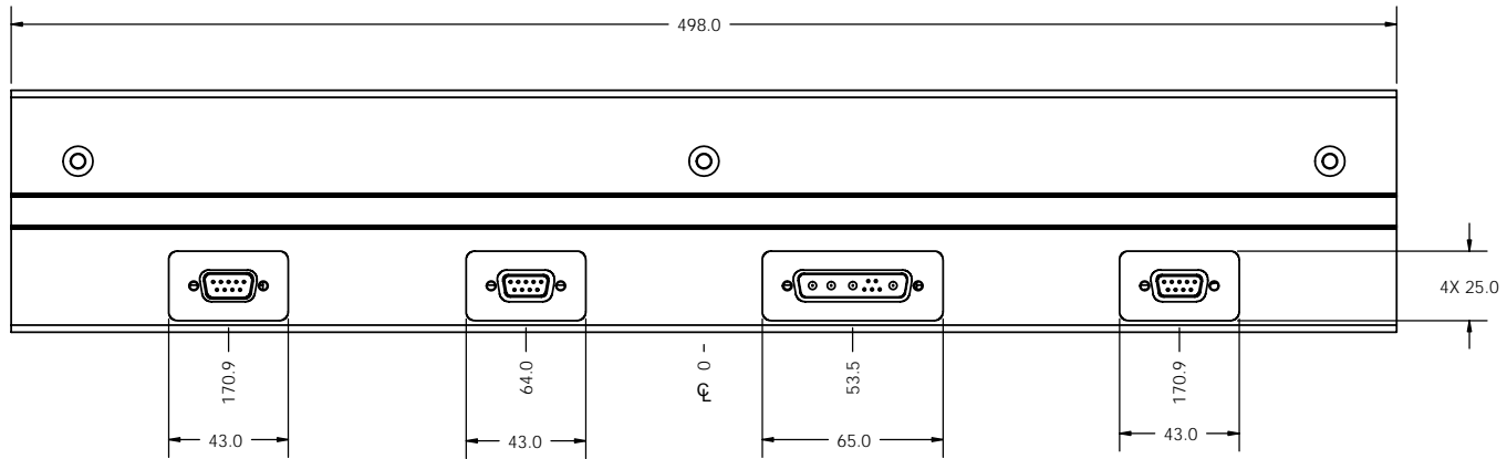
VIEW B-B ROTATED 90° CW SCALE 1 : 2 SEE ELECTRICAL ICD FOR CONNECTOR DETAIL
