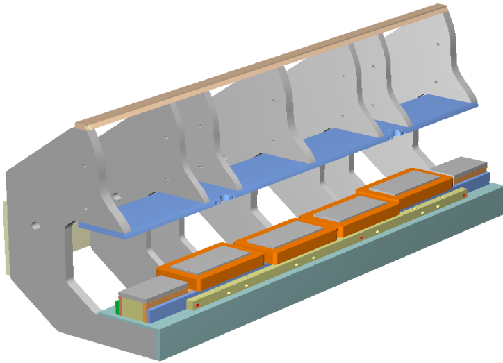
Fig. 2. Magnet pod with permanent magnets and control coils.
