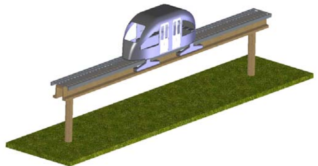
Fig. 4. Vehicle concept for M3 System with ODU girders.
