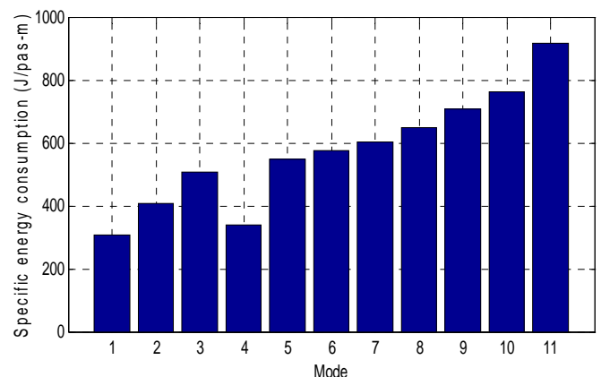
Specific energy use in J/pas-m for different Modes:
