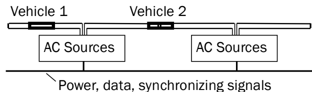
Figure 10. Inductive power transfer system.
