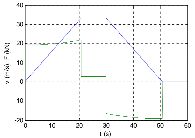
Figure 6. Speed (m/s) and LSM force (kN) vs. t (s) for 1 km trip.
