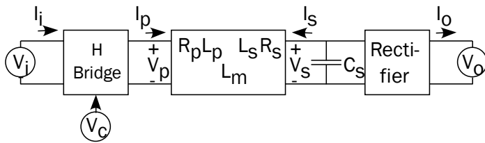
Figure 9. Model of IPT module.
