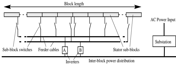
Figure 5. Leap-frog sub-block switching scheme.
