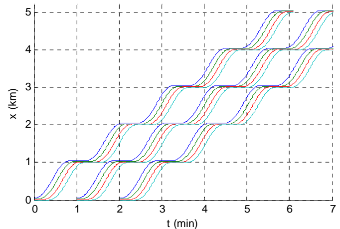
Fig. 2. Distance vs. time plots for clusters of four vehicles making a stop every 1 km.
