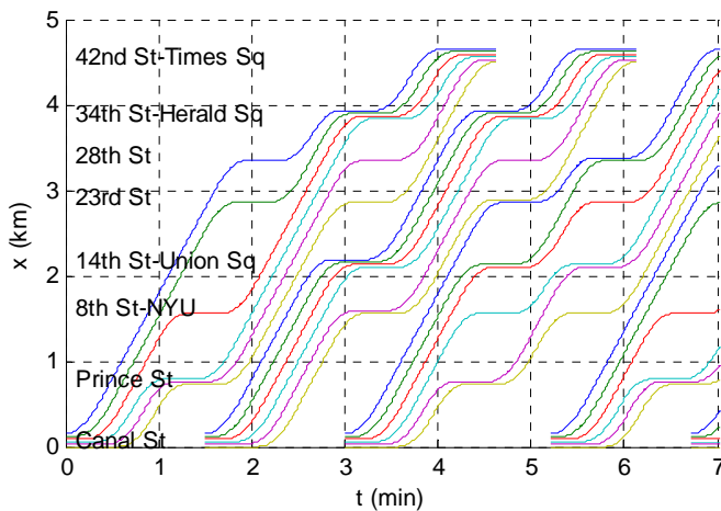
Figure 3. Distance vs. time for one group of clusters and part of an additional group.
