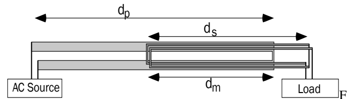
Figure 7. Inductive power transfer module.
