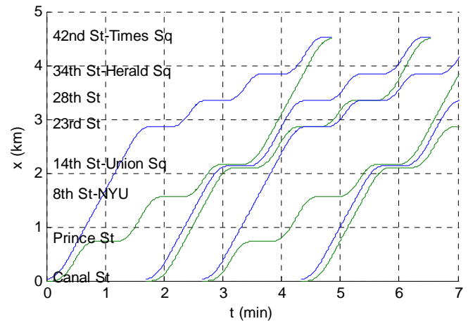
Figure 4. Distance vs. time for two groups of clusters.
