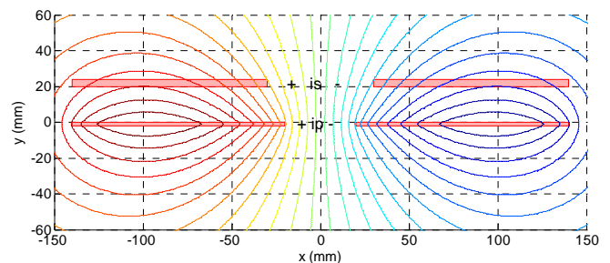
Figure 8. Magnetic field in vicinity of IPT conductors with current only in primary.
